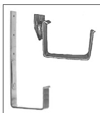
Box gutter bracket/hanger, galvanized steel (N = nose i.e. hook, S = spring i.e. tongue)
